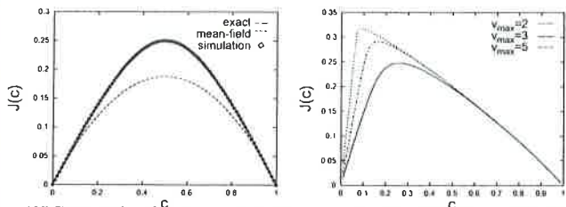
FIG. 6. The fundamental diagram in the NaSch model for (a) V_{max} = 1 and (b) V_{max} > 1 , both for p = 0.25 . The data for all V_{max} > 1 have been obtained through computer simulations.
